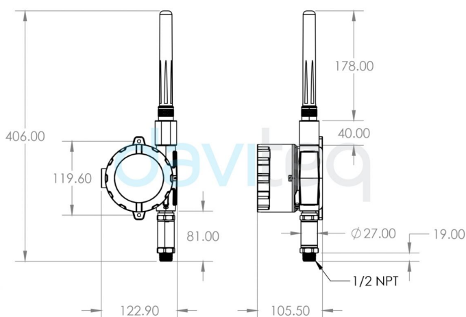
DIMENSION DRAWING OF WSNBEX-PPS (Unit: mm)
